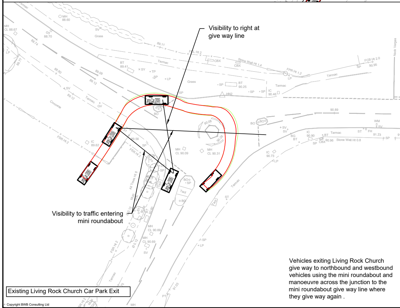
HGV Swept Paths
